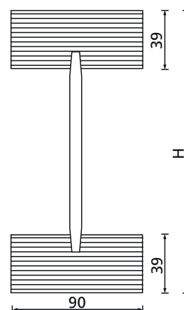
Hunton I-bjelken SJ90
