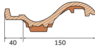
Figur 15: Hollander V 2/3 stein
