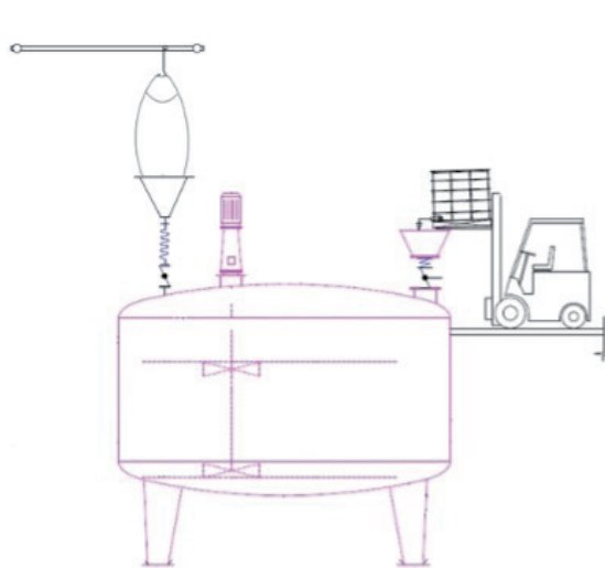
Figure 1: Production process
