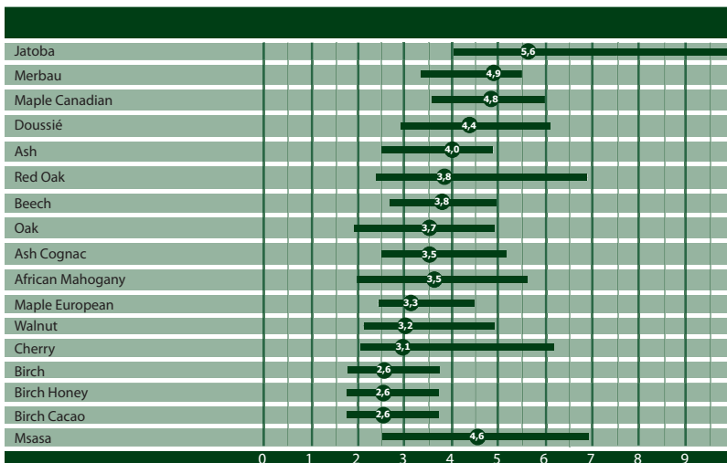
Wood floors, Brinell Hardness (BHN), EN1534
