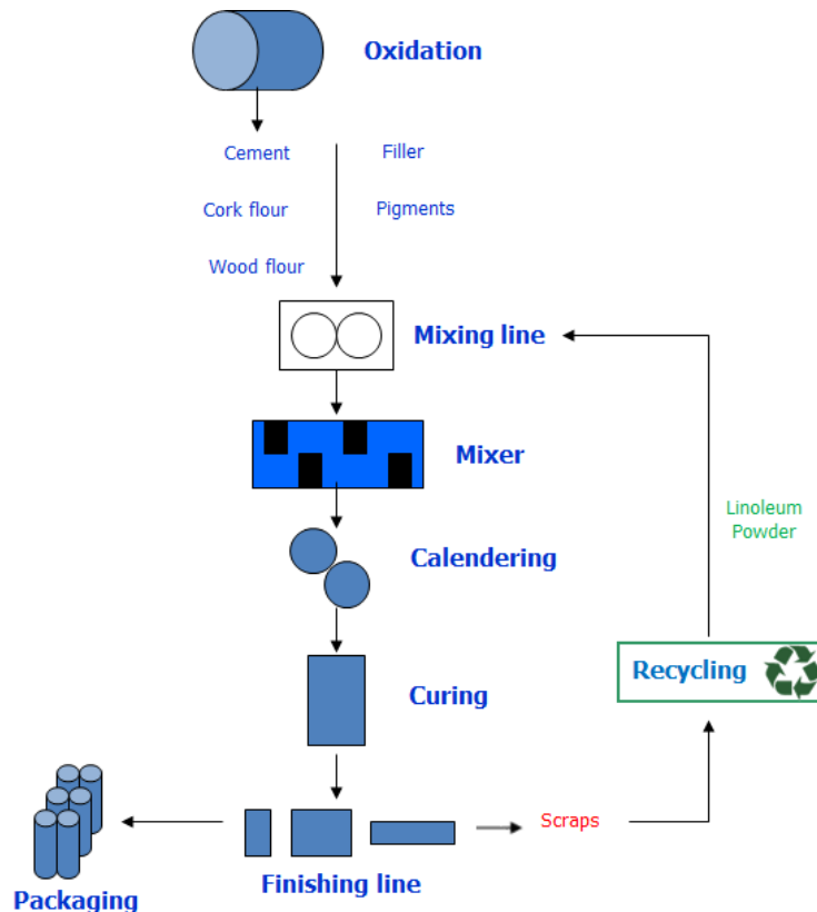
Figure 3: Diagram of production process
