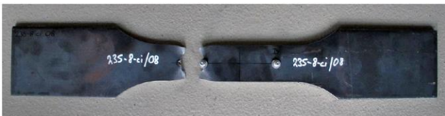
Specimen for fatigue test
