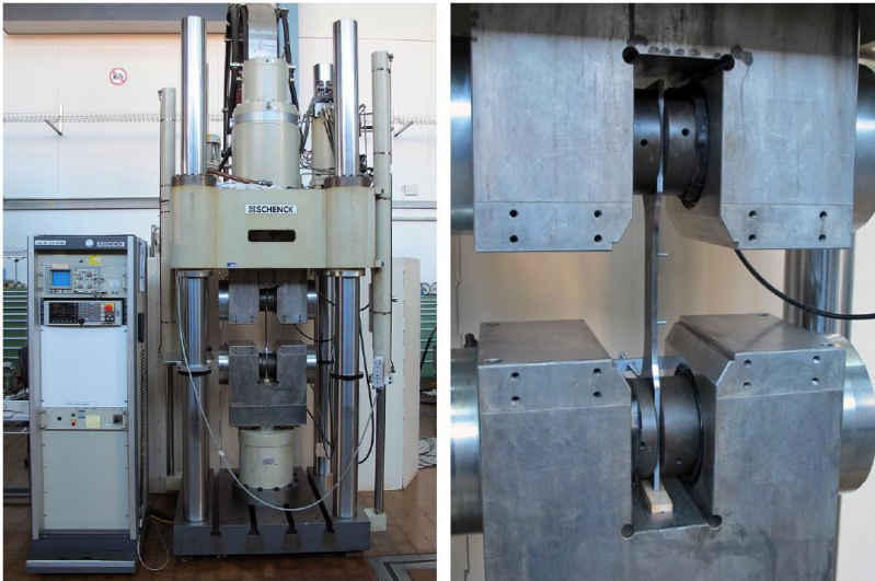
Test facility for fatigue test
