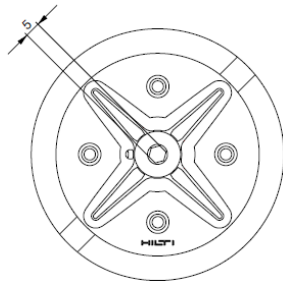
X-FCM-M grating disc
