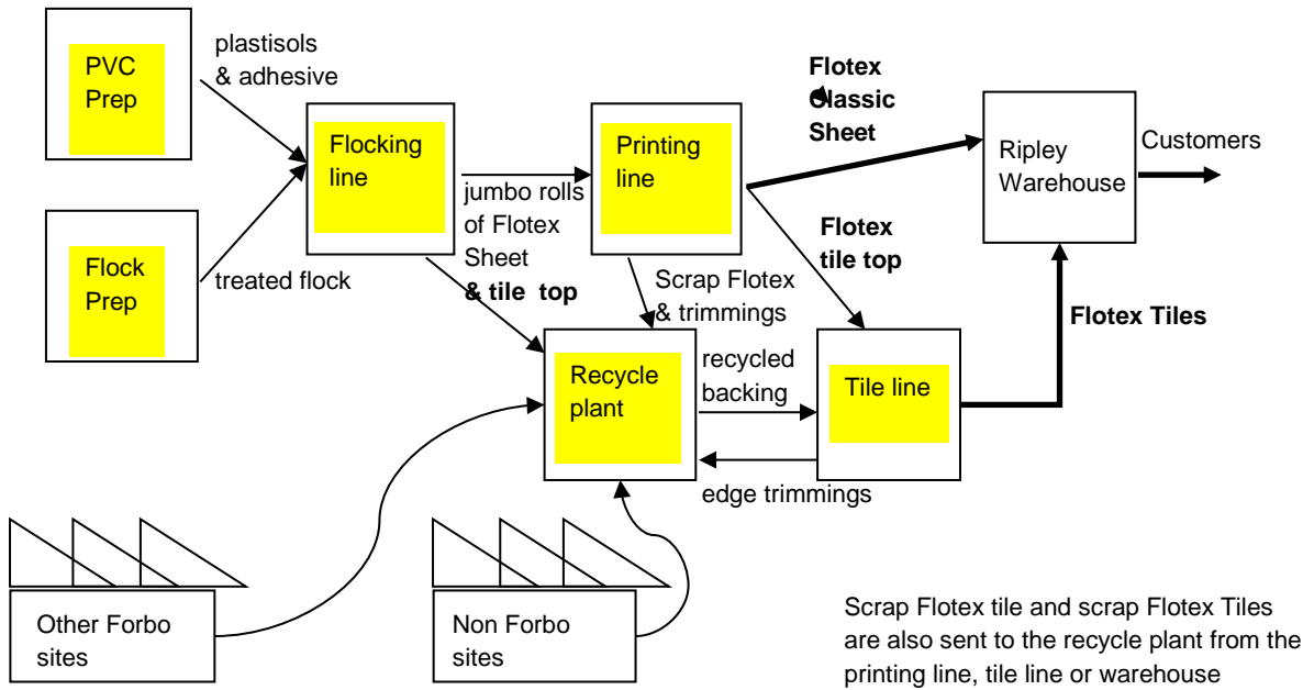
Figure 2 : Schematic manufacturing of Flotex tile
