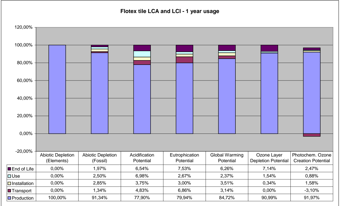
Figure 4: relative contribution of each process stage to each impact category for Flotex tile for a one year usage.
