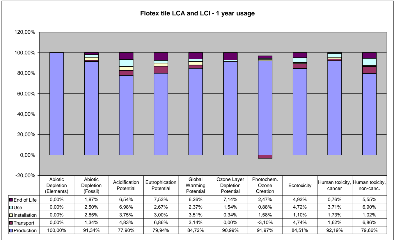
Figure 5: relative contribution of each process stage to each impact category for Flotex tile for a one year usage.
