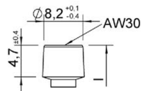
Cylinder head
