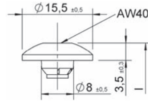
Truss head - design: with and without cutter ribs
