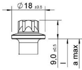
Hexalobular head
