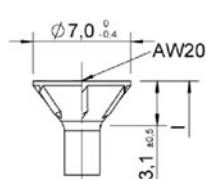
Countersunk head 75° – design with and without raise
