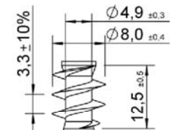
Underhead thread
