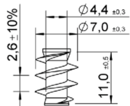
Underhead thread
