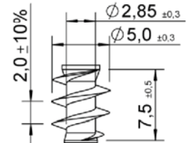
Underhead thread
