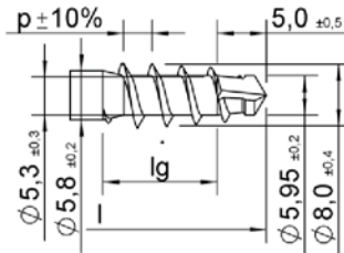
ASSY plus special Design with p = 5.6
