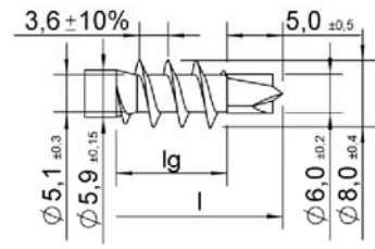
ASSY plus 3.0
