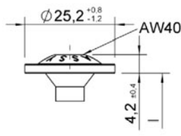
Large washer head
