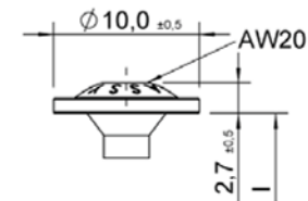
Alternatively at countersunk heads: modification of the shank at drilled head
