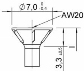
+Countersunk head 75° – design with and without raise
