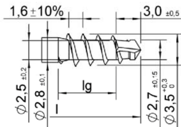
ASSY plus special
