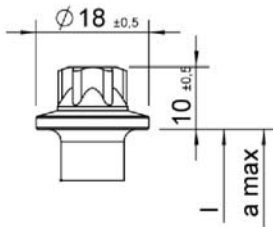
Hexalobular head
