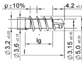
ASSY plus special Design with p = 2.2 und 3.1
