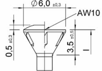
Woodwork head – design with and without raise
