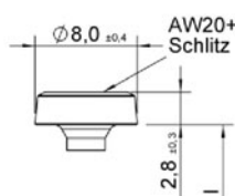
Elmo head
