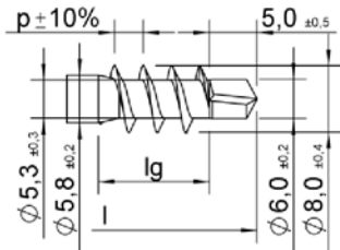
ASSY plus Design with p = 5.6
