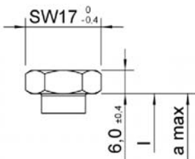
Kombi hexagonal head
