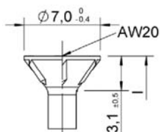
Countersunk head 75° – design with and without raise
