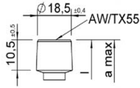
Cylinder head
