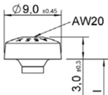
Pan head
