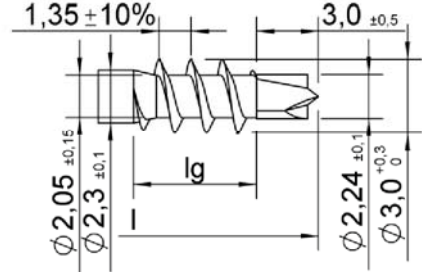
ASSY plus 3.0
