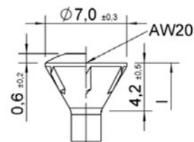
Woodwork head – design with and without raise
