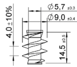
Underhead thread
