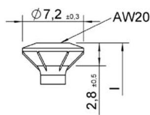
FBS-head
