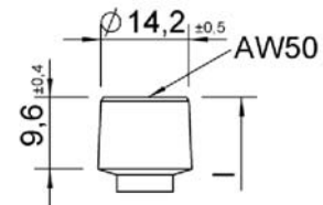
Cylinder head
