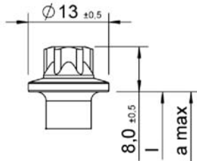
Hexalobular head
