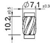
Shank cutter
