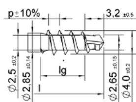
ASSY plus special Design with p = 1.8 and 2.6
