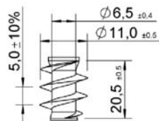
Underhead thread
