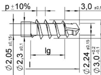
ASSY plus special Design with p = 1.35 and 1.9
