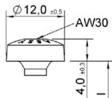
Pan head
