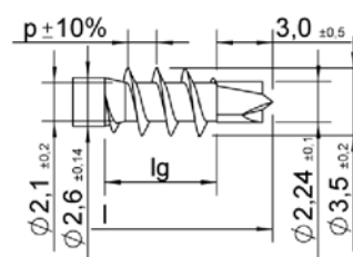
ASSY plus 3.0 Design with p = 1.6 and 2.2
