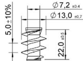
Underhead thread
