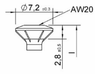
FBS-head
