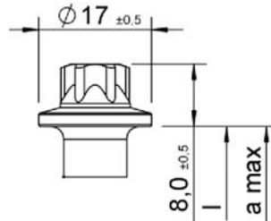
Hexalobular head
