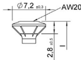
FBS-head
