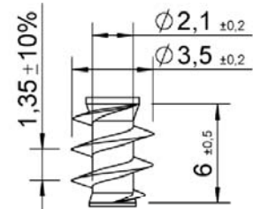
Underhead thread
