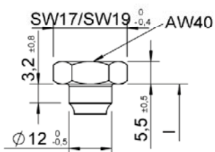
Kombi hexagonal head
