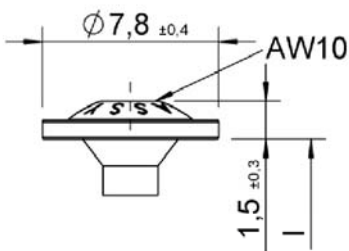
Back panel screw head
