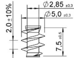
Underhead thread
