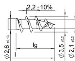
ASSY coarse thread Design with and without ring respectively mating thread
