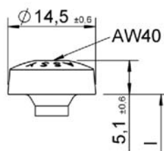
Large washer head
