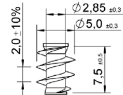
Underhead thread
