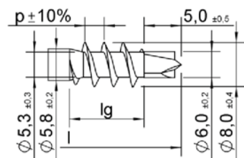
ASSY plus 3.0 Design with p = 5.6
