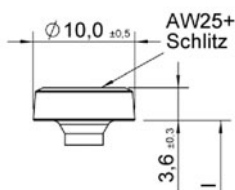
Elmo head
