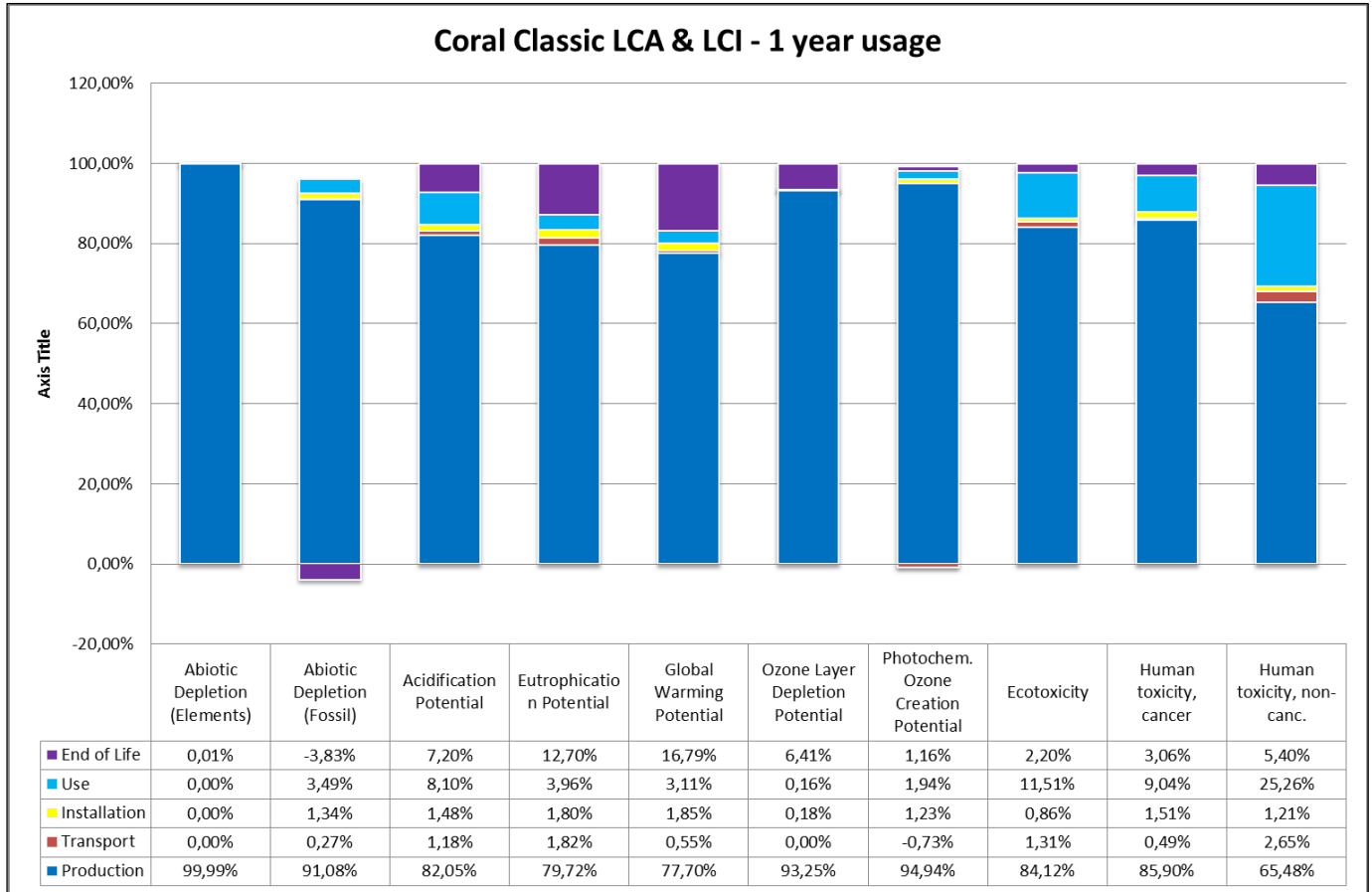
Figure 4: relative contribution of each process stage to each impact category for Coral Classic for a one year usage.
