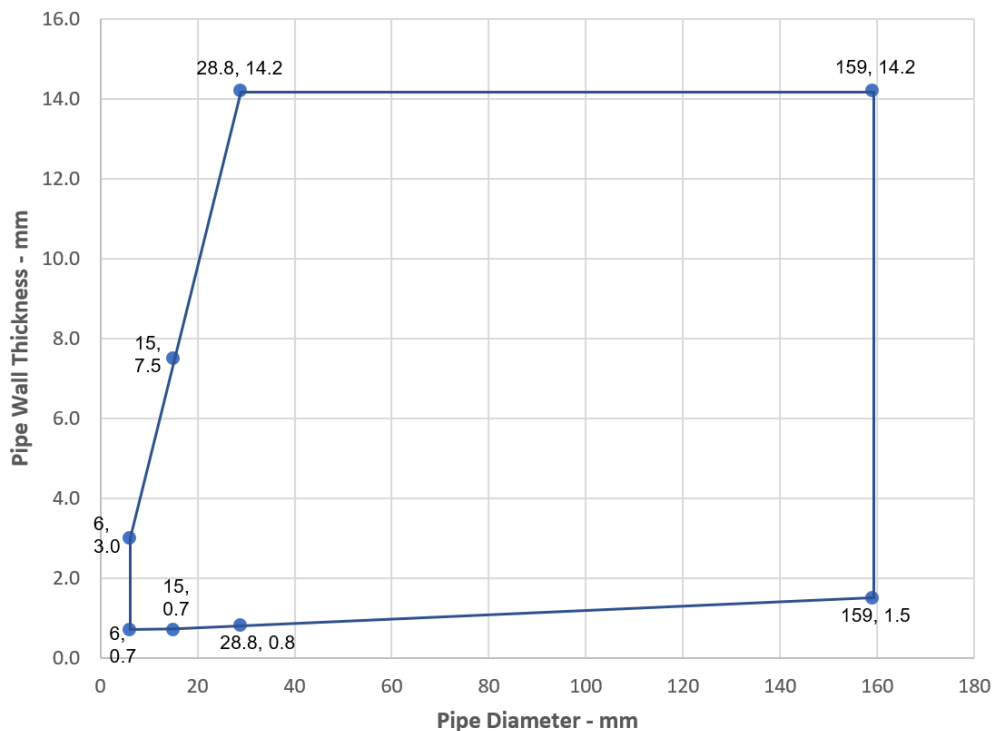
Copper or Steel Pipes with Phenolic Foam Insulation - C/C
