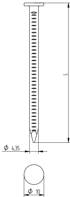
Eurofast ISPC Nail A2 \phi 4,35
