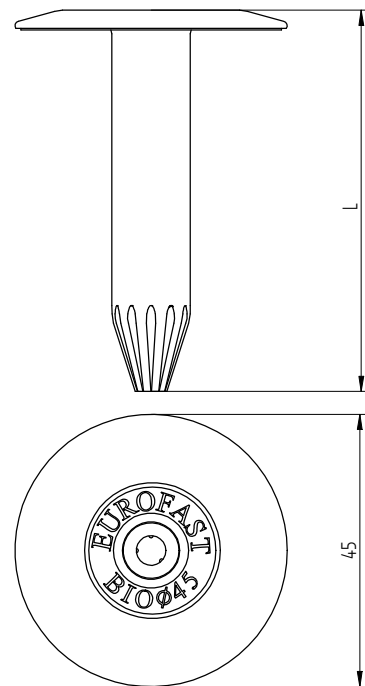
Eurofast BIO-45-L
