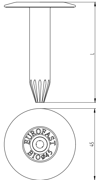
Eurofast BIO-45-L
