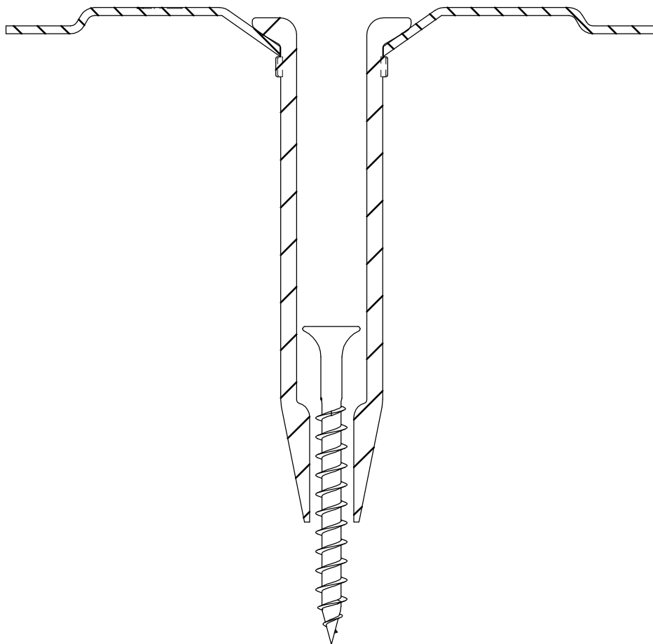
Eurofast EDS-H 5,0 x L
