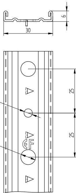
Eurofast EDF-BAR-FB
