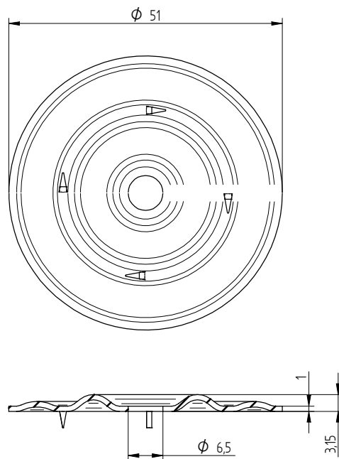
Eurofast DVP-EFB-51NS
