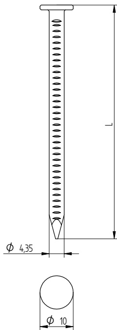
Eurofast ISPC Nail \phi 4,35
