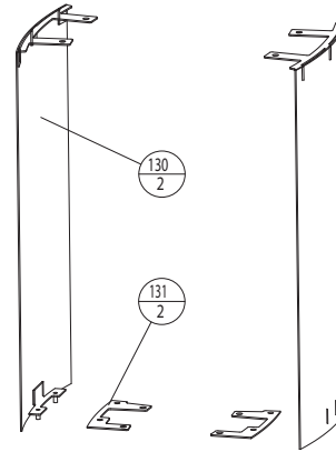
350954 Steel decor Side Low Jøtul F 270 GP
